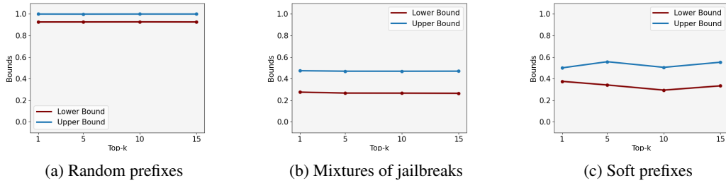
Figure 12: Ablation study showing variations of average certification bounds with Top-k parameter.
