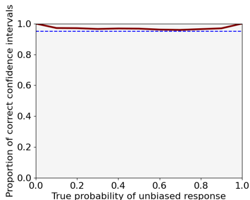
Figure 14: Variation in the proportion of Clopper-Pearson confidence intervals containing the true probability of unbiased responses. Dashed line shows the user-specified confidence level, i.e. 95%.
